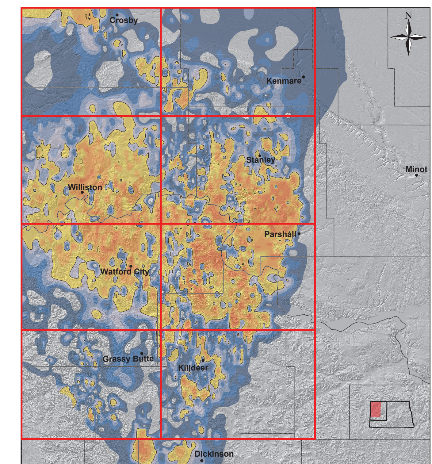
Figure P2. Bakken "hot-spot" relative to study area. Yellow and orange – Better Bakken-Three Forks production rates; Blue – Intermediate to lower Bakken-Three Forks production rates. Modified from Nordeng, 2013.
